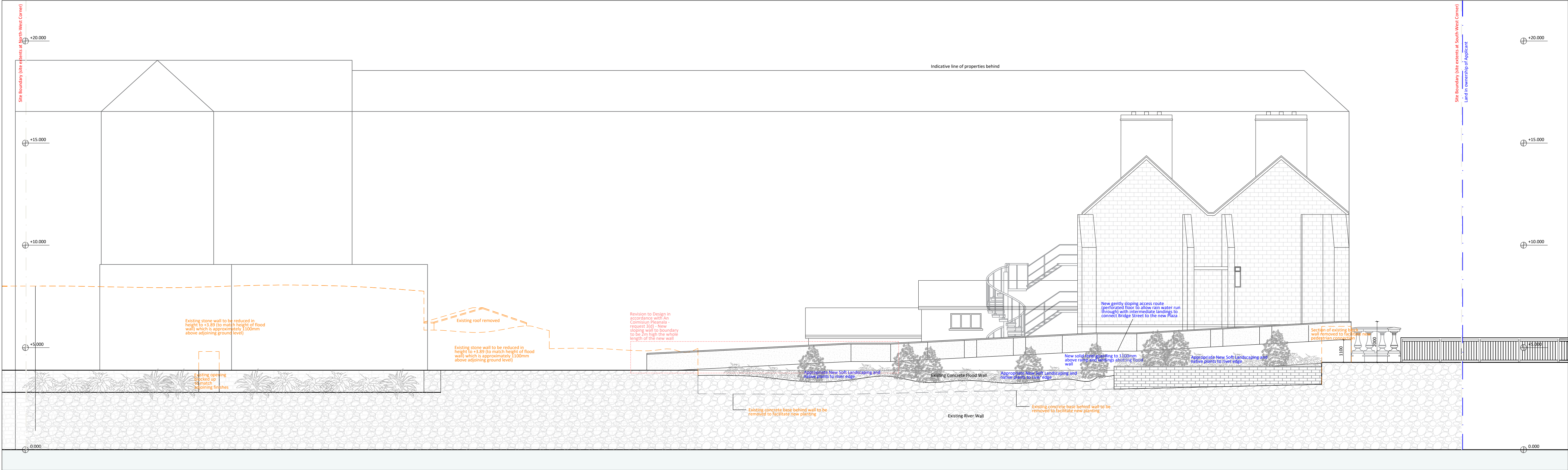
01 Section A-A As Proposed (Elevaiton to Riverside) Scale: 1:100
